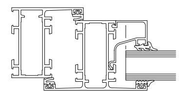
Lateral section outward opening
