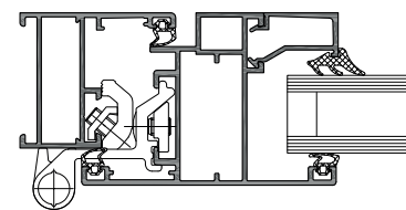
Lateral section with glazing bead
