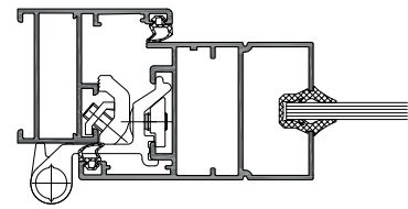
Lateral section without glazing bead
