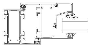
Lateral section inward opening
